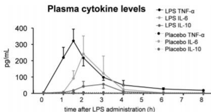
FIGURE 3 | Plasma levels of the cytokines TNF- \alpha , IL-6, and IL-10 in 30 subjects who received an intravenous administration of lipopolysaccharide (LPS) ( n = 15 ) or placebo ( n = 15 ) at T = 0 . Data are represented as median [IQR].
