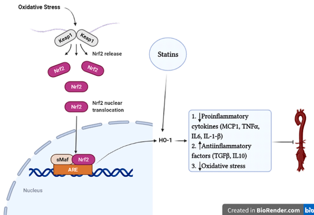
Fig. 2. Effects of statins on Nrf2/HO-1 signaling pathway to reduce AAA development. Nuclear factor erythroid 2-related factor 2 (Nrf2), Heme oxygenase-1 (HO-1), Kelch-like ECH-associated protein 1 (keap1), antioxidant response element (ARE), small musculoaponeurotic fibrosarcoma proteins (sMAF), monocyte chemo-attractant protein-1 (MCP-1).
