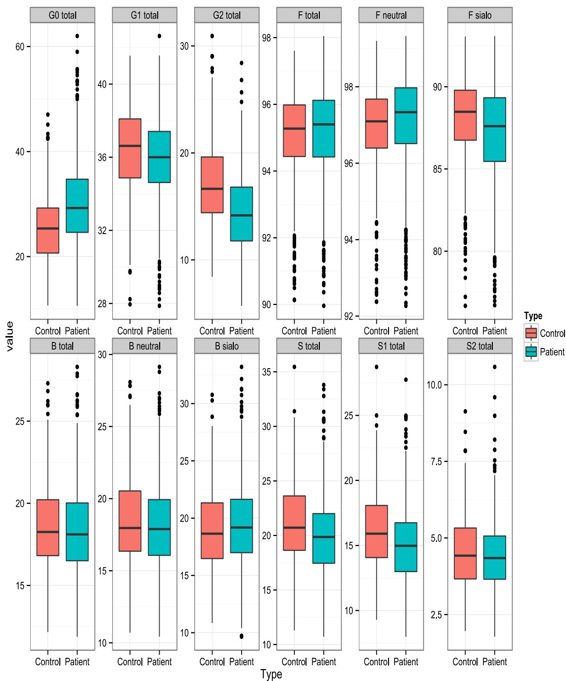
Figure 7. IgG glycome composition in CRC patients and matching controls.
