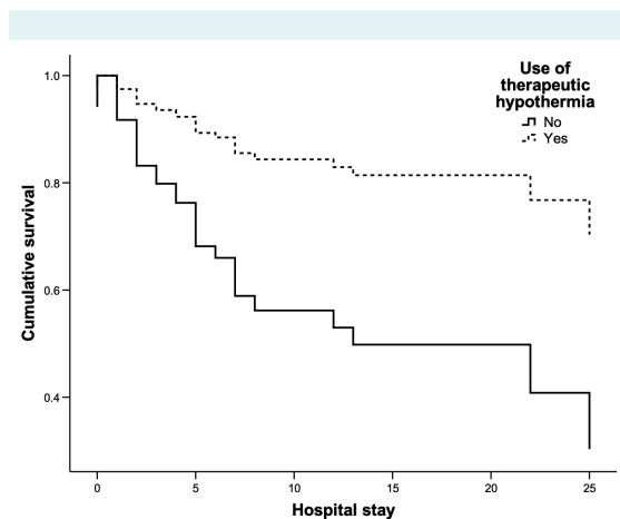
FIGURE 3. Cox proportional hazards model survival curves separated by the use of therapeutic hypothermia.
