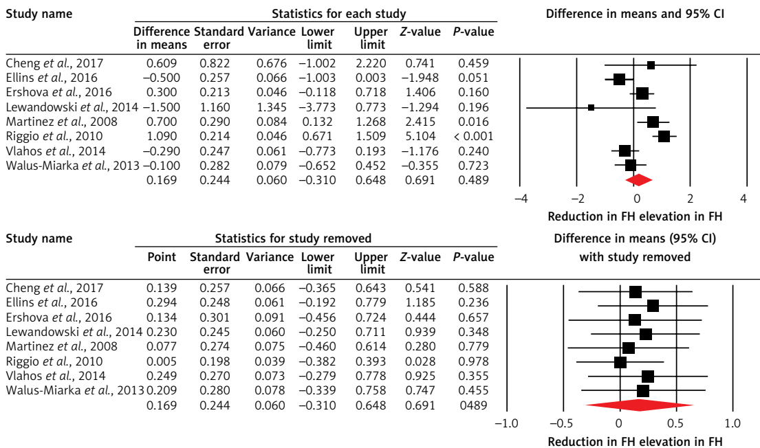
Figure 2. Forest plot displaying weighted mean difference and 95% confidence intervals of pulse wave velocity between patients with familial hypercholesterolemia and unaffected controls. Lower plot shows leave-one-out sensitivity analysis
