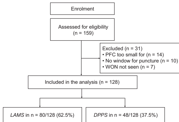
Figure 2 Study flowchart
